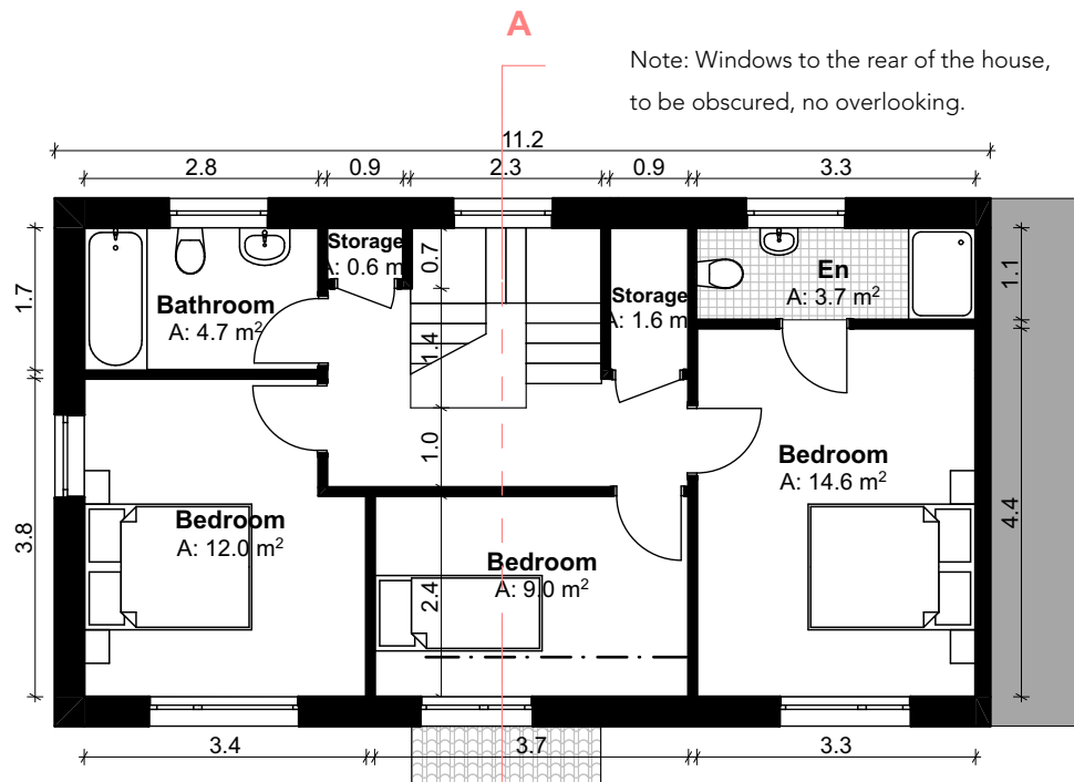
First Floor SCALE 1:100 GFA: 59.64 m 2
