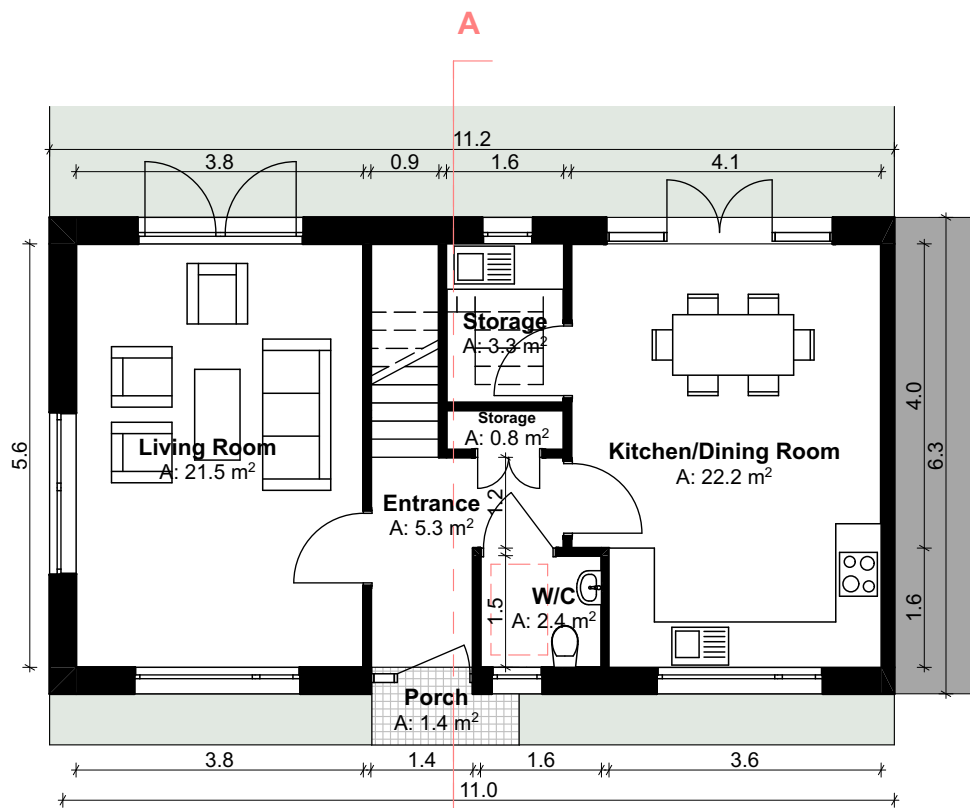
Ground Floor SCALE 1:100 GFA: 59.64 m 2
