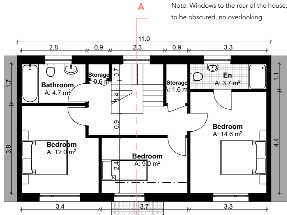
First Floor SCALE 1:100 GFA: 59.64 m 2
