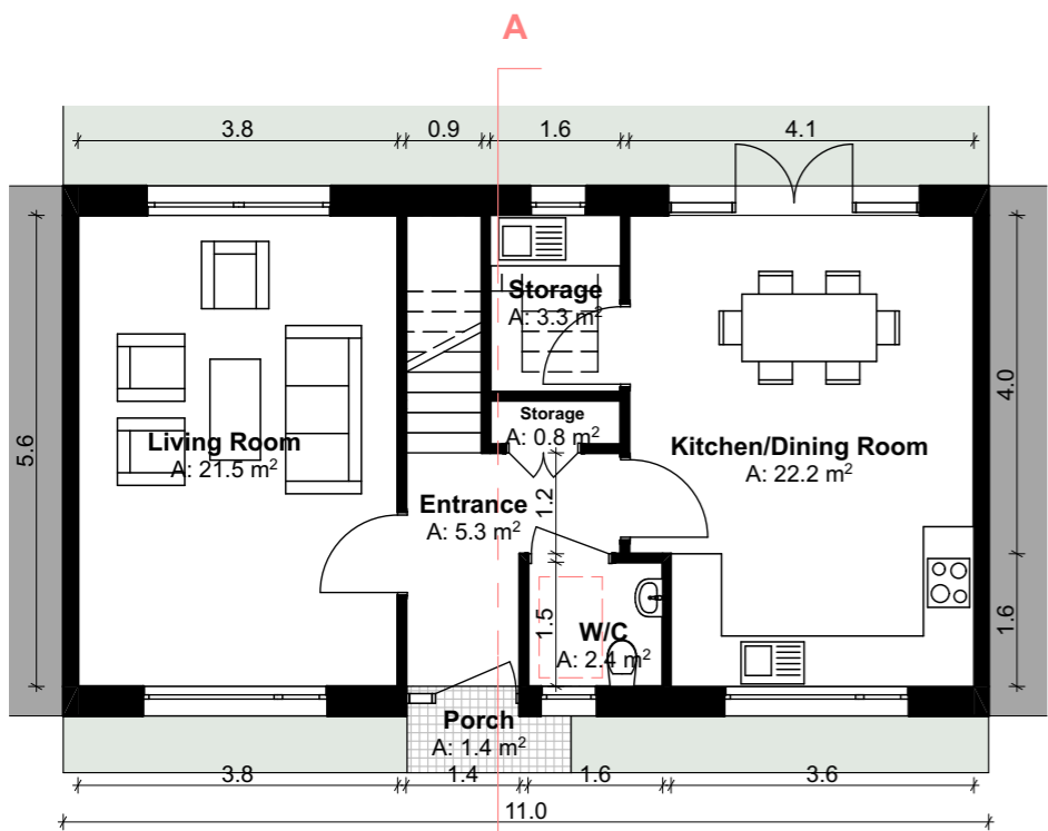
Ground Floor SCALE 1:100 GFA: 59.64 m 2
