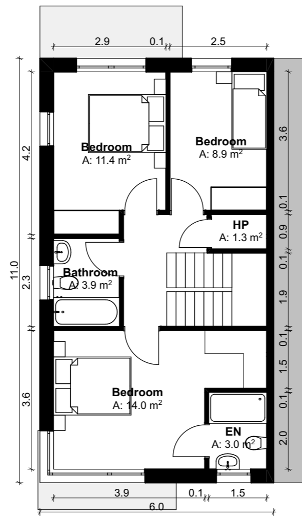
First Floor SCALE 1:100 GFA 56.46 m 2
