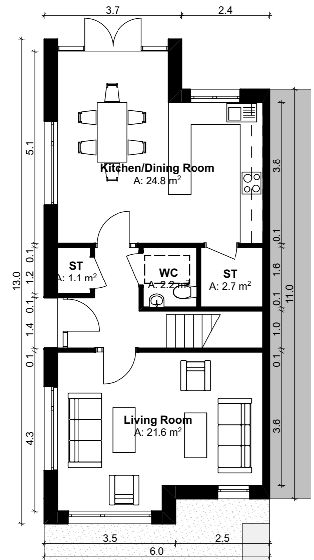
Ground Floor SCALE 1:100 GFA 62.68 m 2
