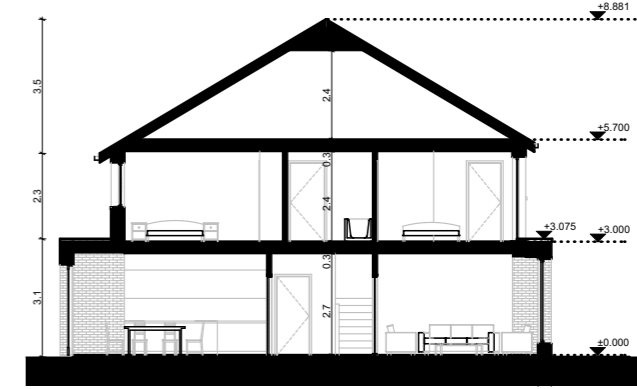
Building Section SCALE 1:200
