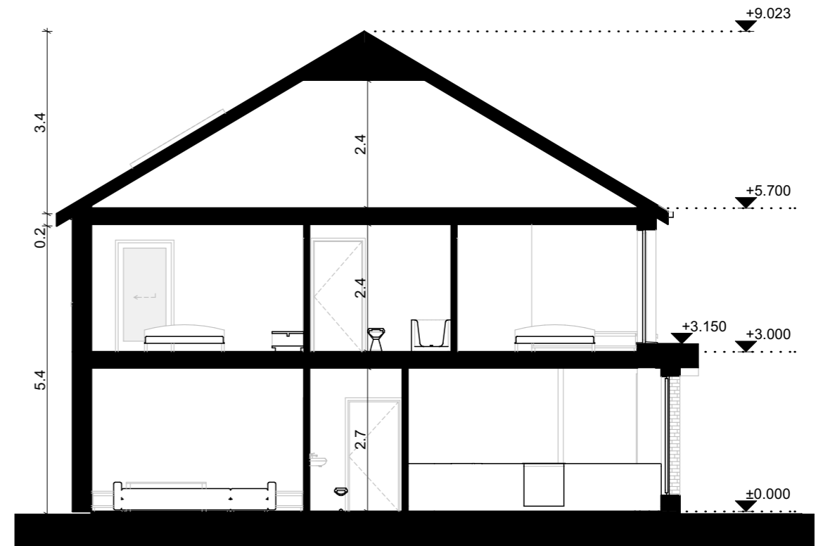
Building Section SCALE 1:100
