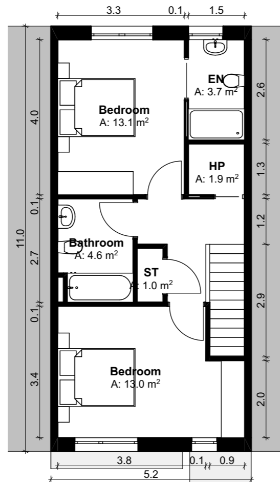
First Floor SCALE 1:100 GFA: 49.53 sqm
