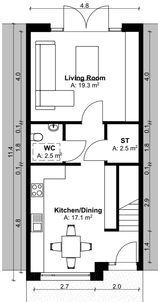
Ground Floor SCALE 1:100 GFA: 50.53 sqm
