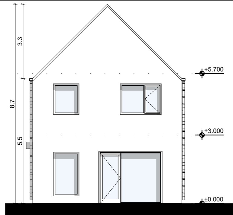
Back Elevation SCALE 1:100
