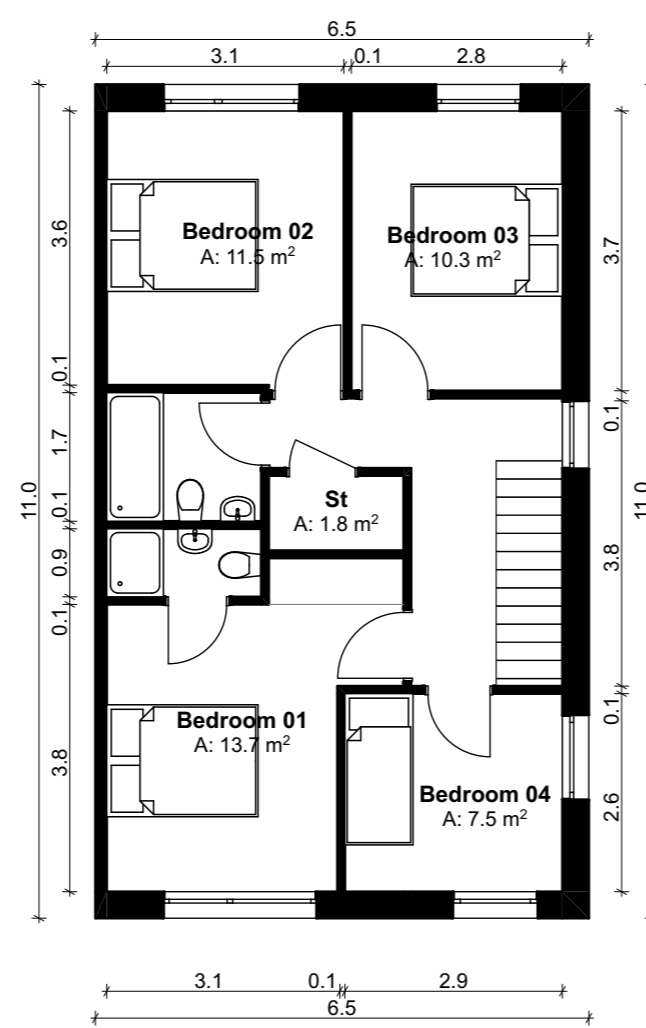
First Floor SCALE 1:100 GFA: 62.21 sqm
