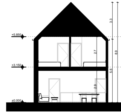
Building Section SCALE 1:200
