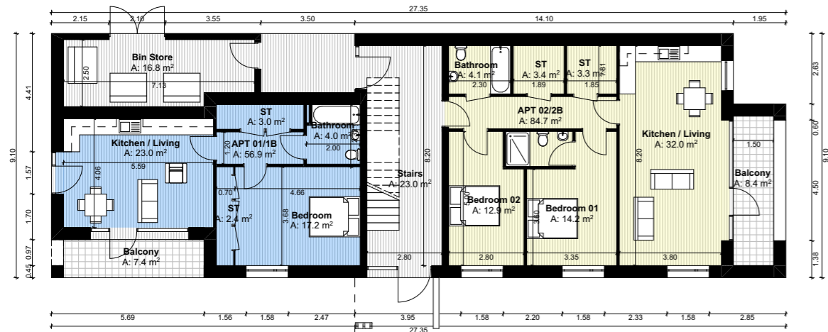
Ground Floor Plan SCALE 1:200
