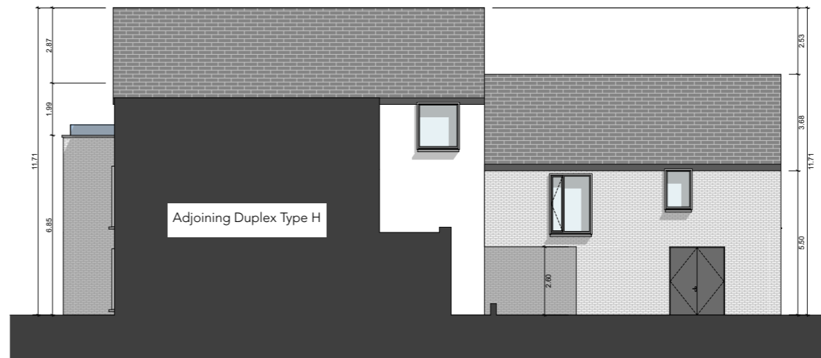
Rear Elevation SCALE 1:200
