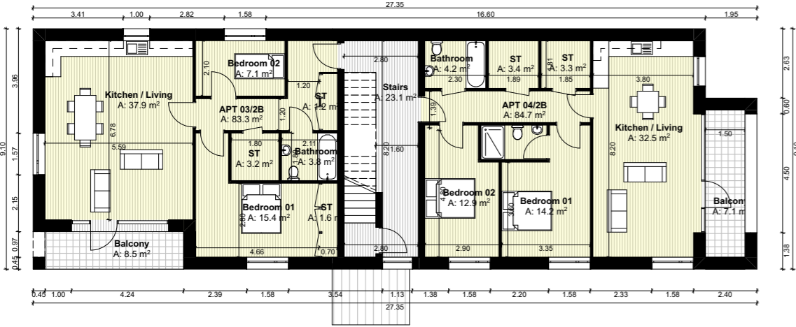
First Floor Plan SCALE 1:200
