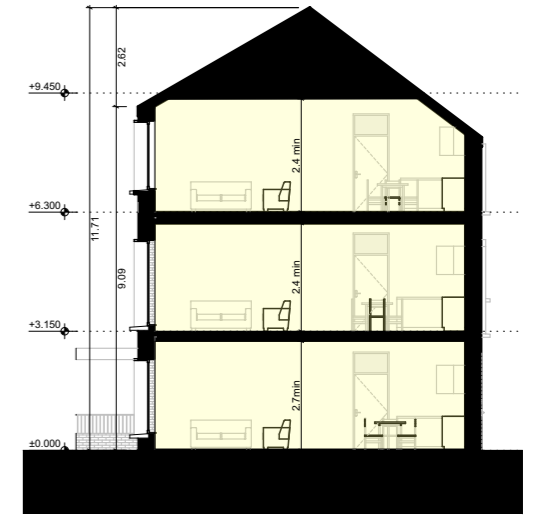
Typical Cross Section SCALE 1:200
