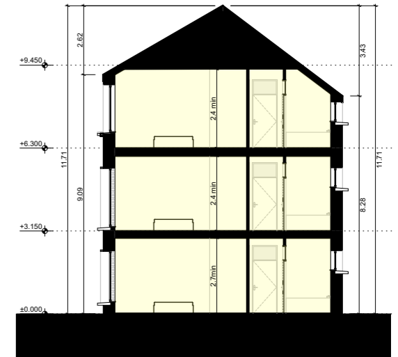
Typical Cross Section SCALE 1:200
