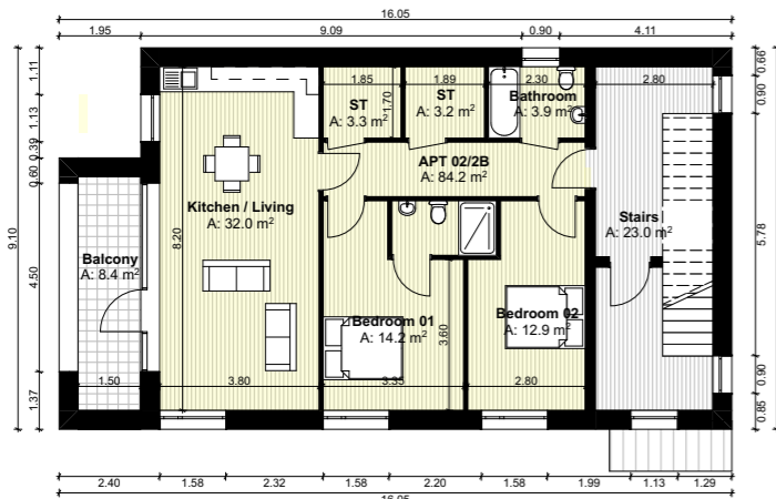
First Floor Plan SCALE 1:200
