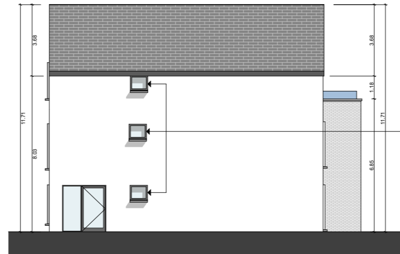
Rear Elevation SCALE 1:200
