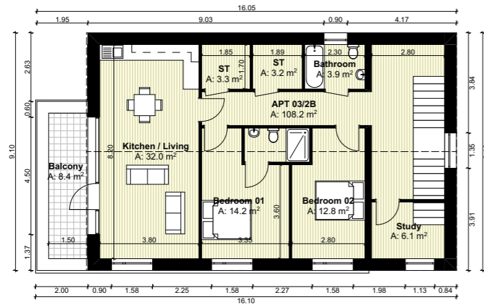
Second Floor Plan SCALE 1:200
