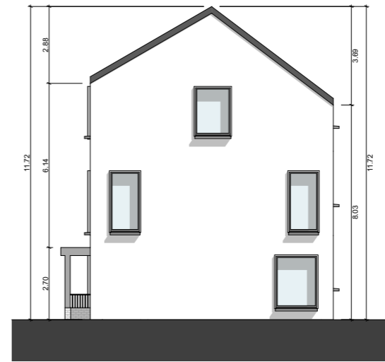
Side Elevation SCALE 1:200
