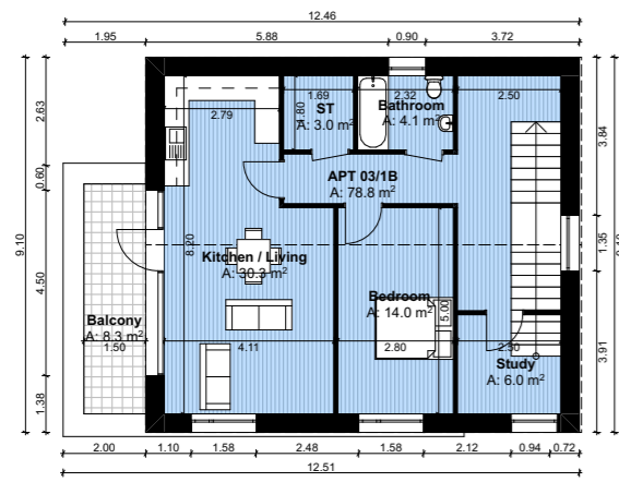
Second Floor Plan SCALE 1:200
